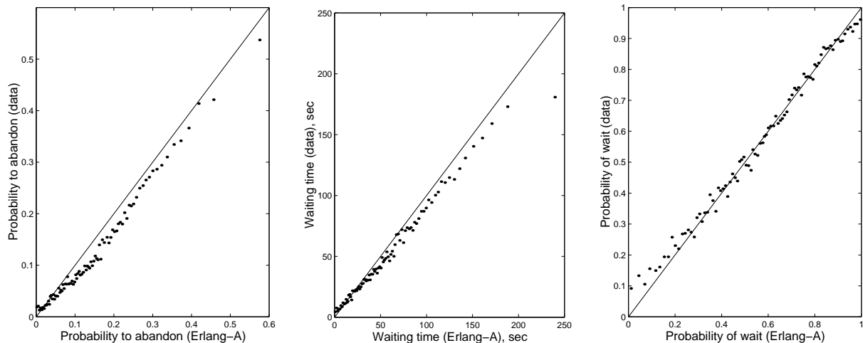
Figure 8: Erlang-A formulas vs. data averages
