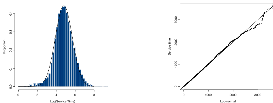
Figure 3: Histogram, QQ Plot of Log(Service Time) (Nov.–Dec.)
