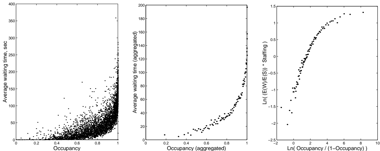
Figure 7: Agents’ occupancy vs. average waiting time
