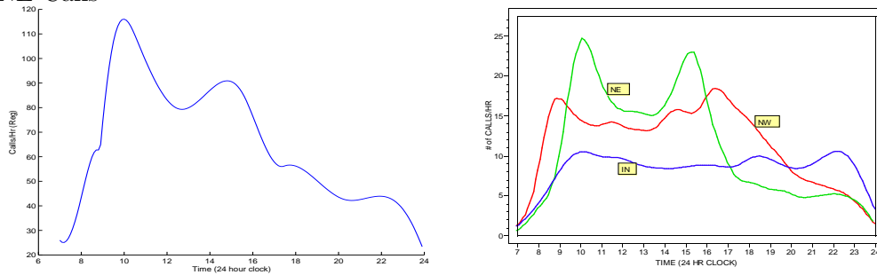
Figure 1: Arrivals in Calls/Hr by Time-of-day, weekdays Nov. - Dec. (Left) PS Calls (Right) IN, NW and NE Calls
