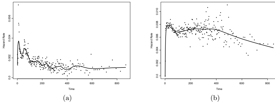
Figure 5: (a) Hazard rate for the time willing to wait for PS calls (Nov.–Dec.) (b) Hazard rate for virtual waiting time (Nov.–Dec.)
