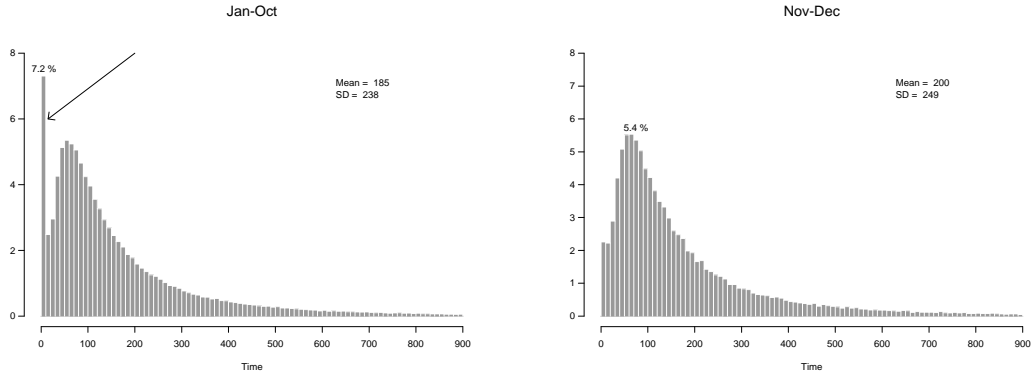
Figure 2: Distribution of service time
