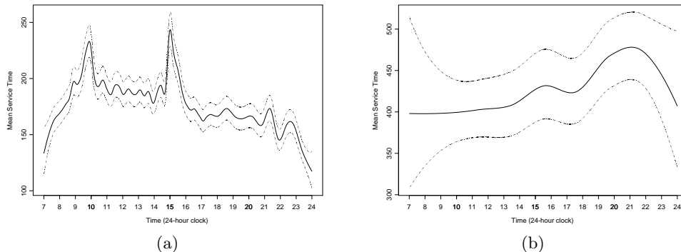
Figure 4: (left) Mean Service Time (PS) versus Time-of-day (95% CI) (right) Mean Service Time (IN) versus Time-of-day (95% CI)
